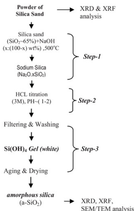
FIGURE 1. The Alkalifusion Route to Synthesize Amorphous Silica.
